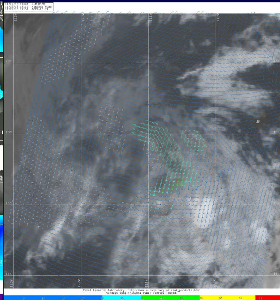
Windsat vector winds – Rick (2015)
