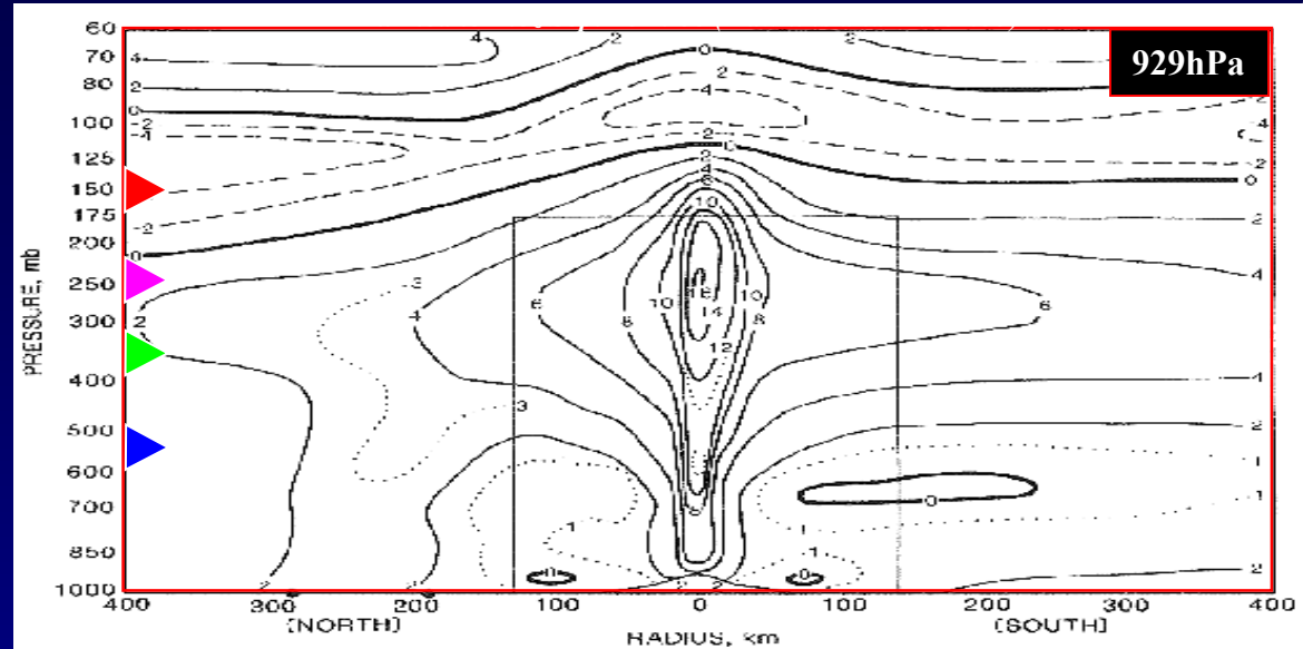
Hurricane Floyd, 14 September 1999, 1200UTC AMSU-A Derived Temperature Anomaly (Storm Center-Environment) Contour Interval = 2°C
