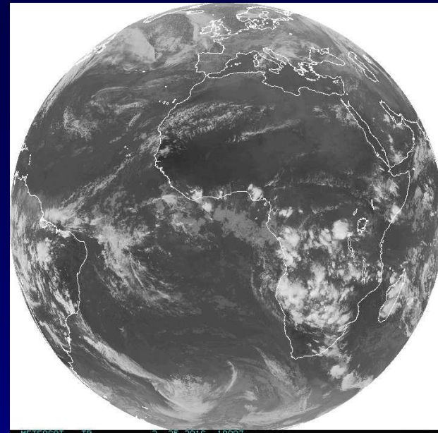
METEOSAT-10 0°
