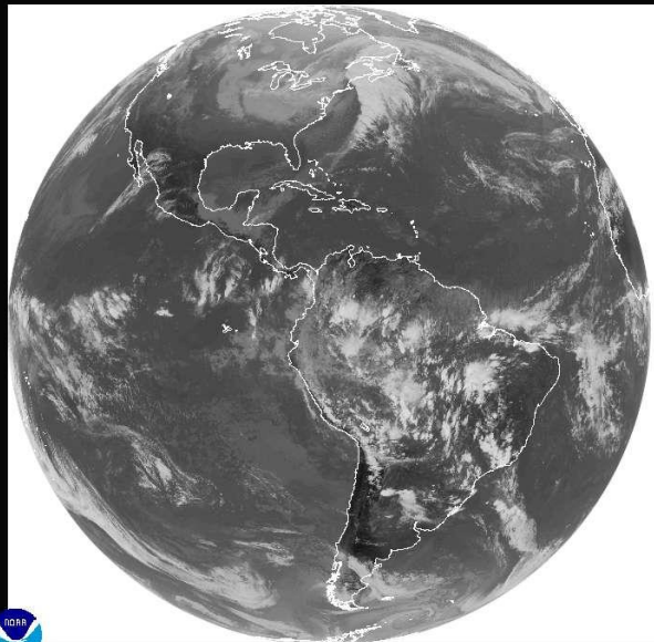
GOES-13 75° W
