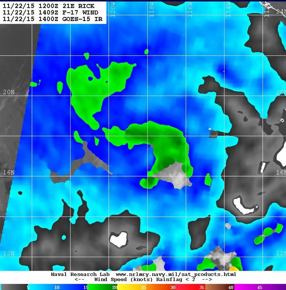
SSM/I Winds – Rick (2015)
