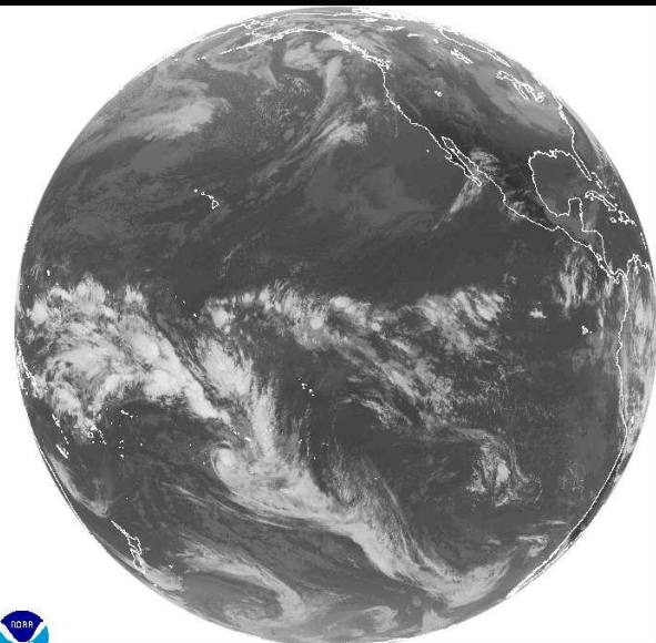
GOES-15 135° W
