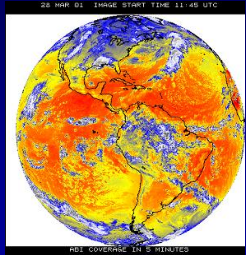
GOES-R
