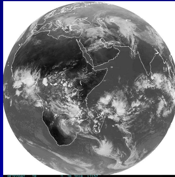
METEOSAT-8 41.5° E
