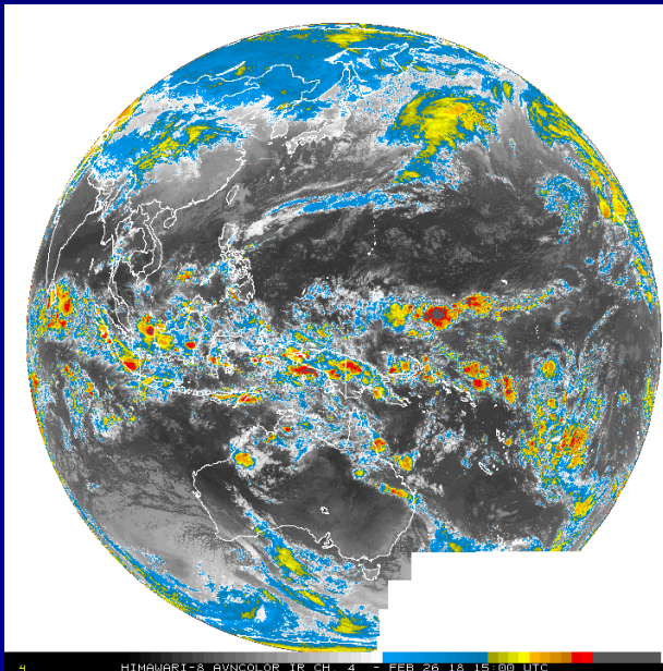
HIMAWARI-8 141° E
